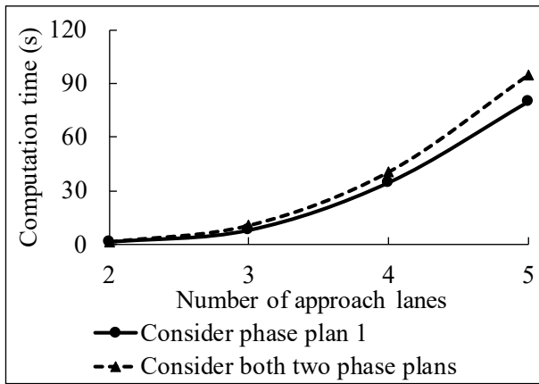
Figure 4. Computation time analysis.
