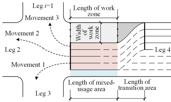
Figure 3. Layout parameters.
