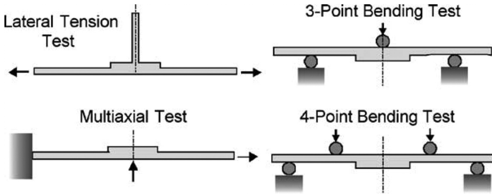
Figure 13. Test setups for characterizing skin-to-stiffener joints which induce stiffener foot tip failure. [253]
