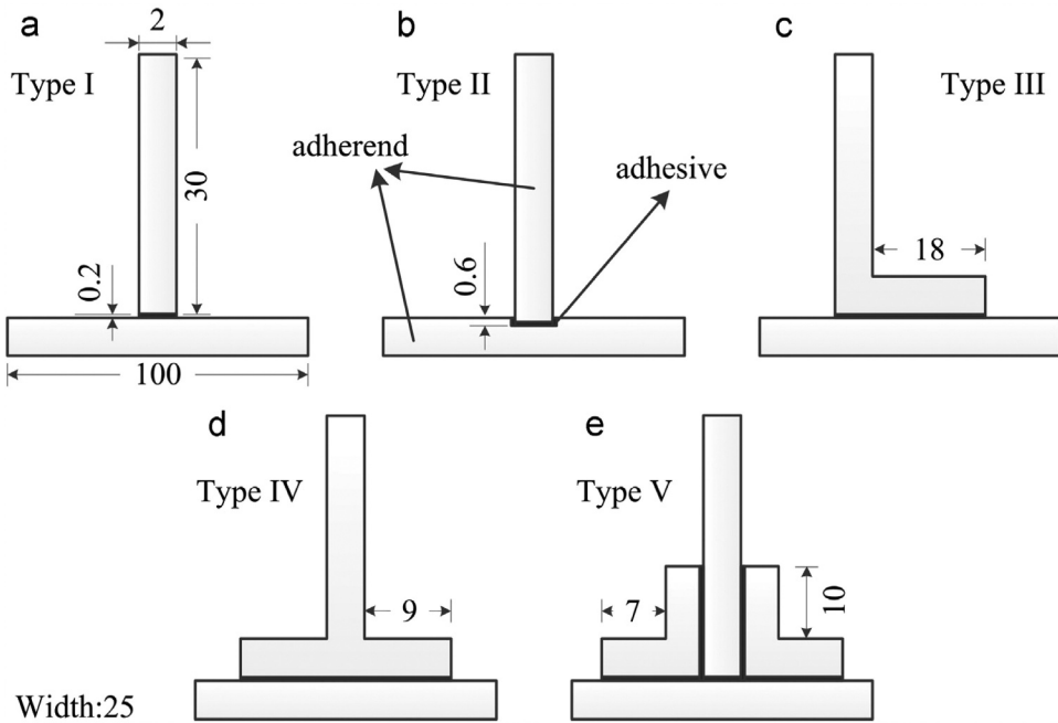
Figure 20. Five skin-to-stiffener joint topologies (dimension in mm). [263]
