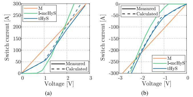
Fig. 6. (a) Forward and (b) reverse ON-state characteristics of four parallel SiC MOSFET, four parallel Si IGBT, and two Si IGBT plus two SiC MOSFET in parallel, derived for T_j = 25 °C, V_{gs} and V_{ge} = +17/-4 V, and R_g = 4 \Omega , and analytically calculated according to (16).
