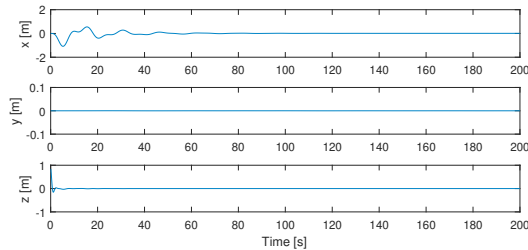
Fig. 5. p_1^n - p_{1d}^n with m=2000t
