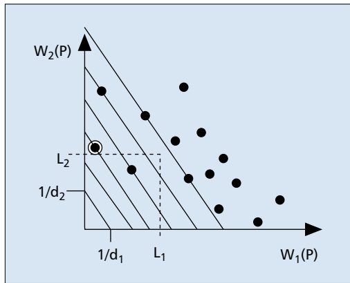
■ Figure 1. Pictorial representation of the search process in Jaffe's algorithm.
