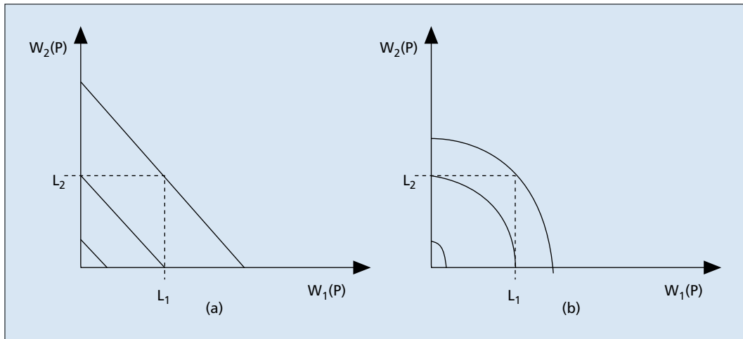
■ Figure 2. Searching for a feasible path by minimizing: a) a linear composite function; b) a nonlinear composite function.
