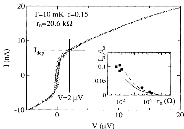
FIG. 2. Current-voltage characteristic of sample B, measured at f = 0.15 and T = 10 \text{ mK} , showing the definition of the depinning current with the 2\text{-}\mu\text{V} criterion. Inset: The ratio of the array depinning current to the array critical current as a function of the junction normal-state resistance. The depinning current is obtained from I - V curves measured at f = 0.15 and T = 10 \text{ mK} . The circles give the results for samples, which have C = 80 \text{ fF} , and the squares the ones for the other samples with C = 160 \text{ fF} . The dashed and solid line present retrapping currents calculated in analogy with single-junction McCumber theory for C = 80 and 160 \text{ fF} , respectively.
