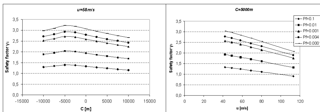
Figure 5: Load safety factor for variations of hurricane parameters
