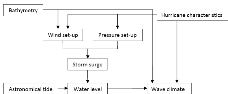
Figure 2: Framework of hydraulic climate (Maaskant, Van Vuren, Kallen, 2009)
