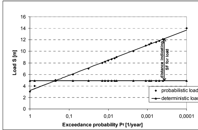
Figure 4: Design and characteristic exceedance curves
