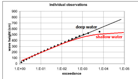
Figure 2: Exceedance curves of wave height in deep and shallow waters
