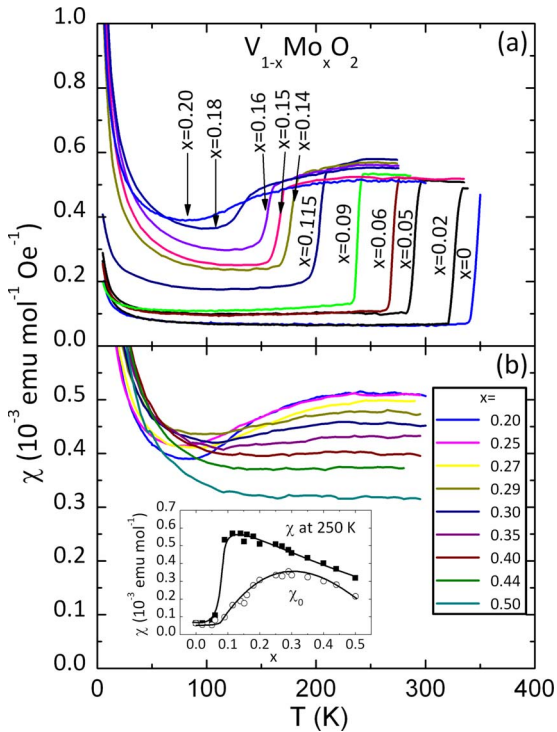
FIG. 3. (Color online) Temperature-dependent magnetic susceptibilities for V_{1-x}Mo_xO_2 (a) for 0 \leq x \leq 0.2 and (b) for 0.2 \leq x \leq 0.5 . The metal-insulator transition temperature is marked by a sudden decrease in susceptibility. Inset (b), \chi at 250 K increases sharply as the I-M transition is crossed on Mo doping, then slowly decreases in the metallic phase between x=0.25 and x=0.50 . The temperature independent part of the low-temperature magnetic susceptibility, \chi_0 , determined from the fits (Fig. 4) is also shown.
