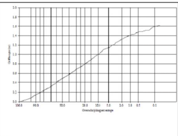
Measured spectrum according to Deltares equipment
