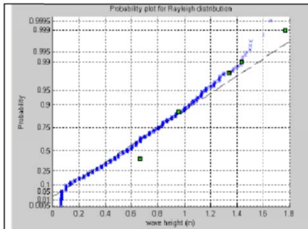
Measured exceedance line with EMS wave logger
