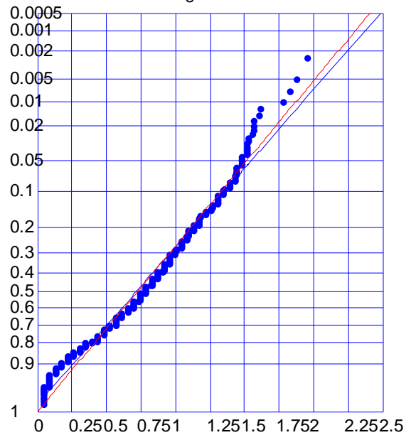
Wave height distribution
