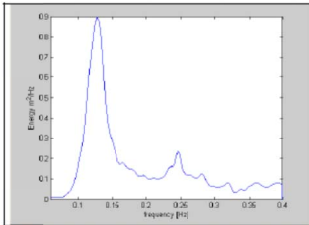
Measured spectrum with EMS wave logger
