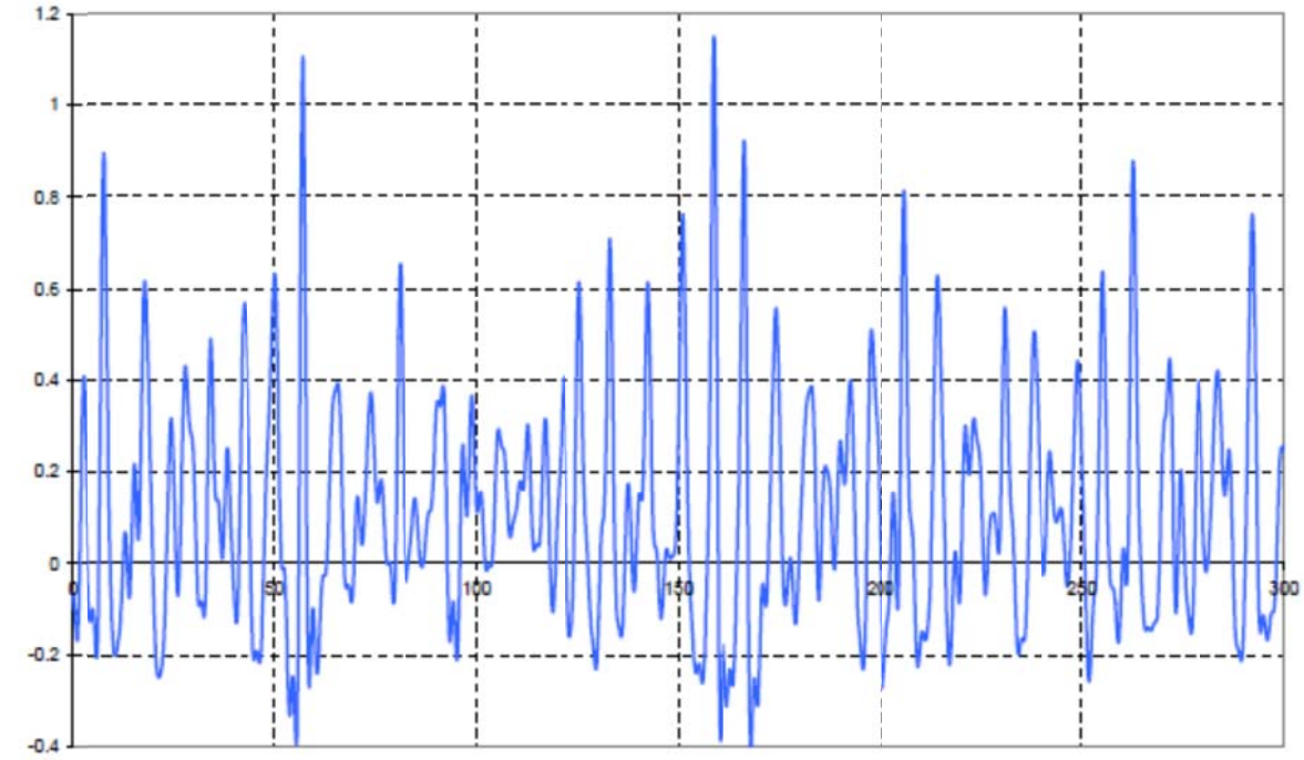
Wave surface elevation measured with Deltares equipment The measurements by EMS wave logger and Deltares Equipment were not at exactly the same location.
