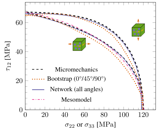
Fig. 22. Biaxial yield envelopes ( \sigma_{22(33)} - \tau_{12} ) obtained with the bootstrapped network ensemble trained on pure stress states plus \theta = 45^\circ and with a single network trained with all values of \theta . The mesomodel envelope is shown for comparison.
