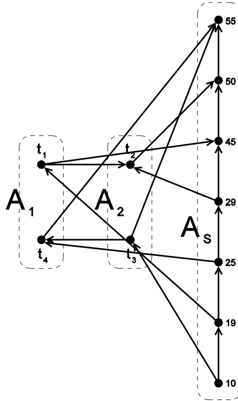
Figure 3. Reducing a temporal coordination problem to a plan-coordination problem.
