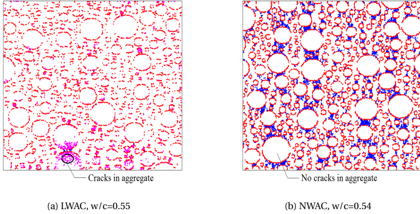
Figure 5.16: Simulated micro-cracks in LWAC and NWAC under a stress of 30% of compressive strength after 30 years (Blue: mortar cracks; Red: bond cracks; Magenta: aggregate cracks)
