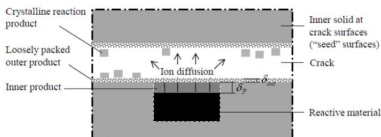
Figure 2.13: Schematic diagram of the self-healing of a micro-crack [14]
