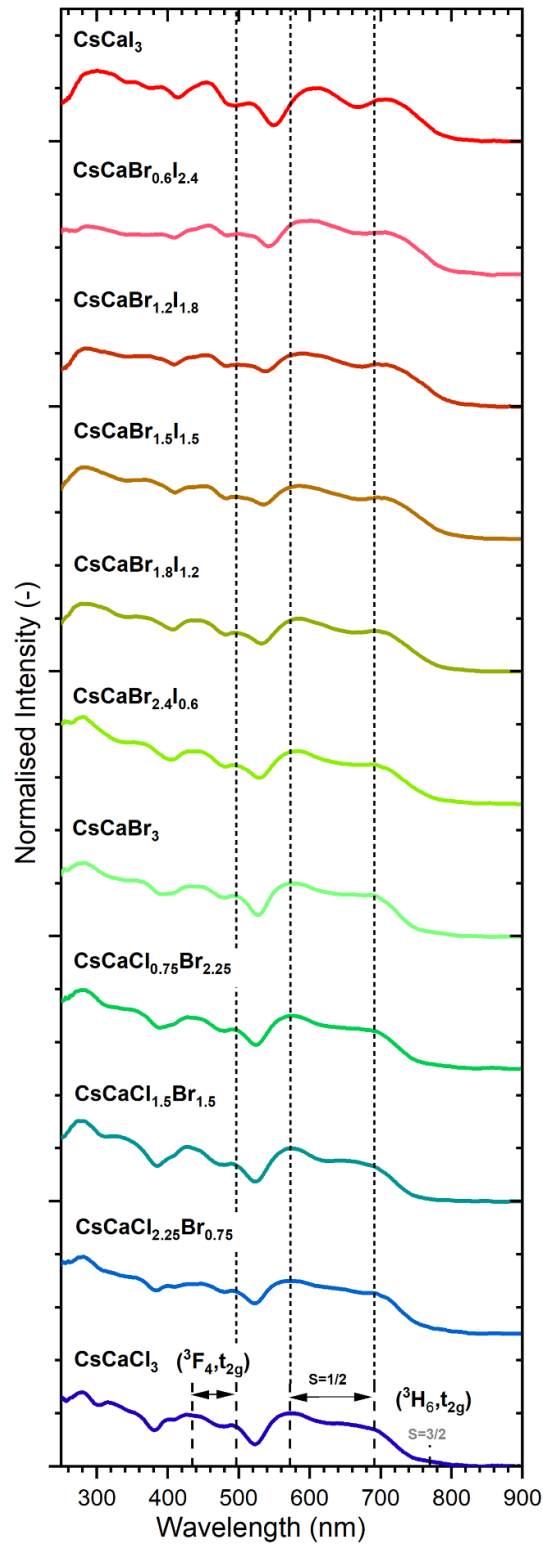
Figure 4. Excitation spectra of the \text{CsCa}(\text{Cl}/\text{Br})_3:\text{TM}^{2+} and \text{CsCa}(\text{Br}/\text{I})_3:\text{TM}^{2+} samples as acquired on {}^2\text{F}_{5/2} \rightarrow {}^2\text{F}_{7/2} emission A at 300 K. The lowest energy 4f^{12}5d^1 -levels are indicated for \text{CsCaCl}_3:\text{TM}^{2+} and undergo a shift towards longer wavelengths upon traversing from \text{Cl} \rightarrow \text{Br} \rightarrow \text{I} .
