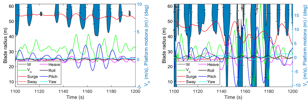
Figure 6. Barge with normal irregular waves (LC1)
