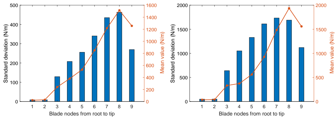
Figure 15. Standard deviation and mean thrust - LC1.
