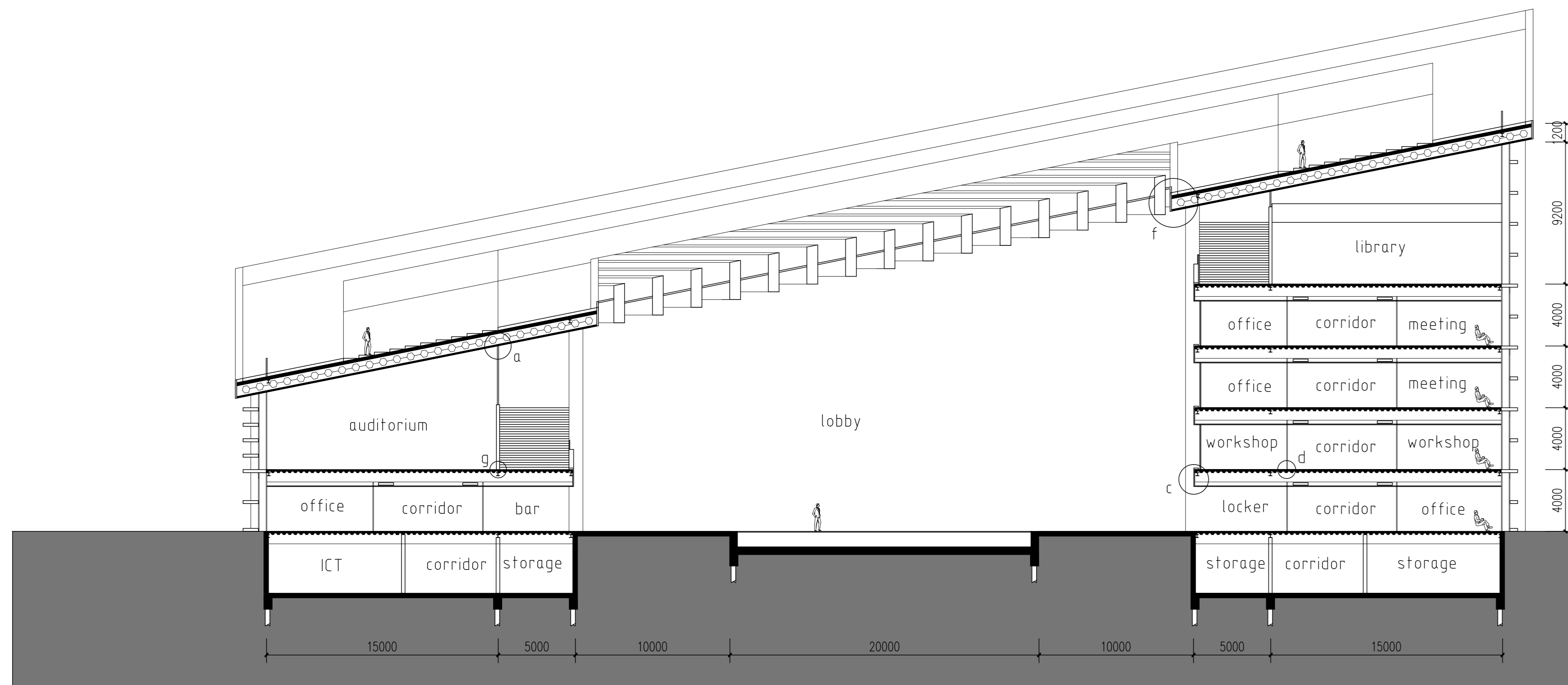
section 1-1 1:200
