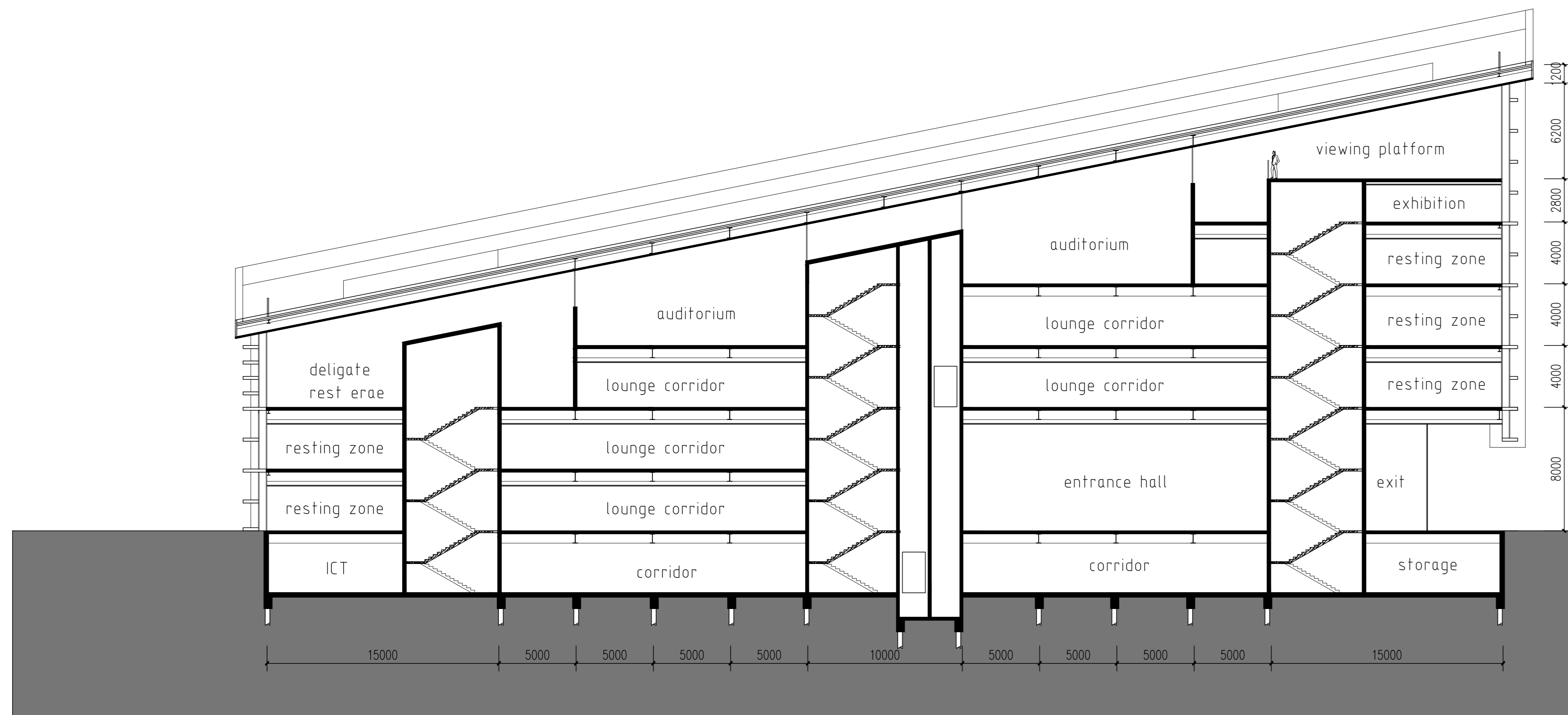
section 3-3 1:200
