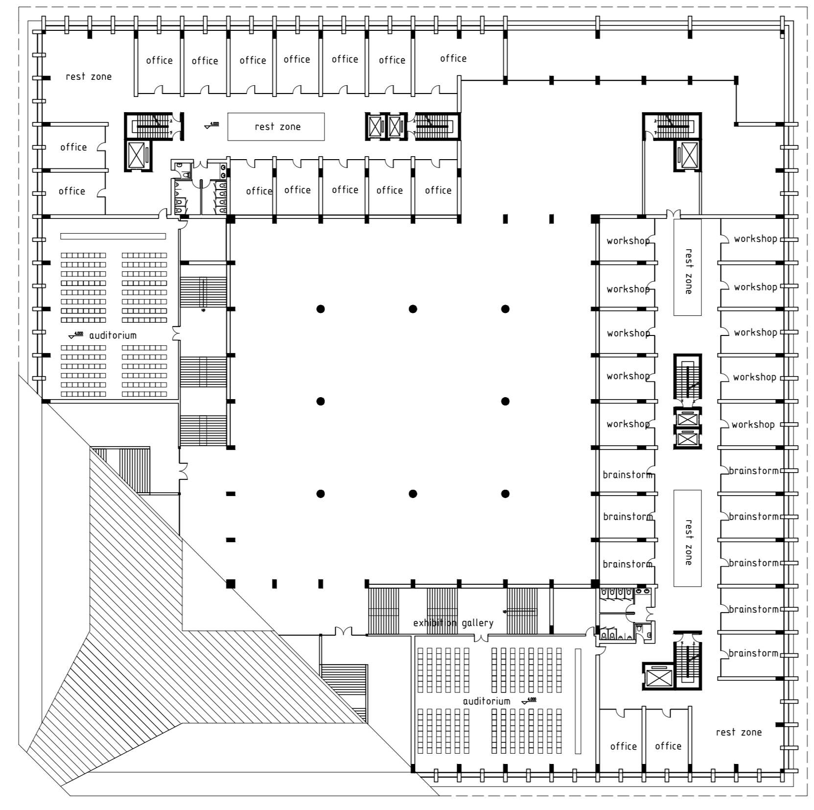
1 plan 1:200
