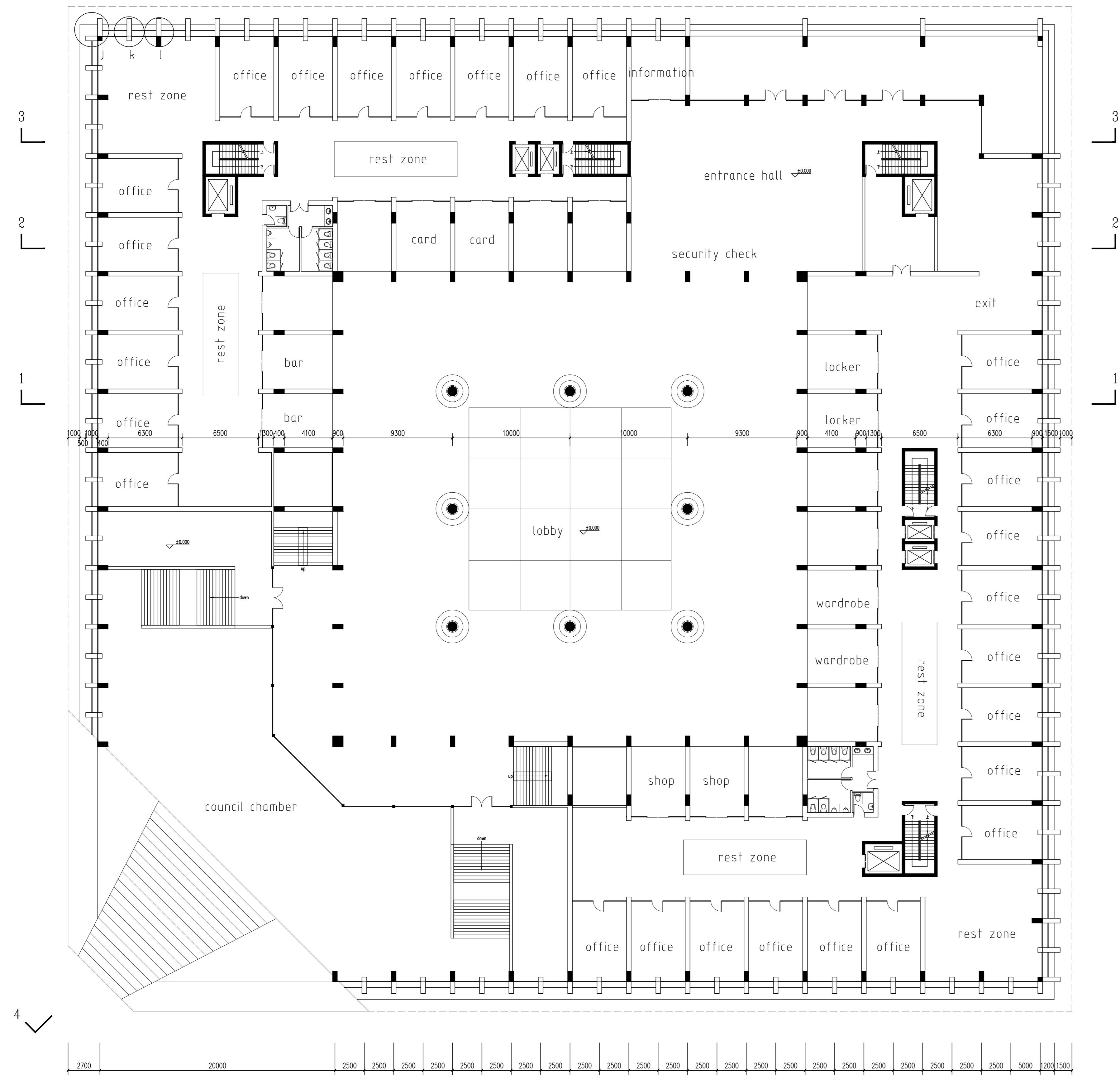
ground plan 1:200
