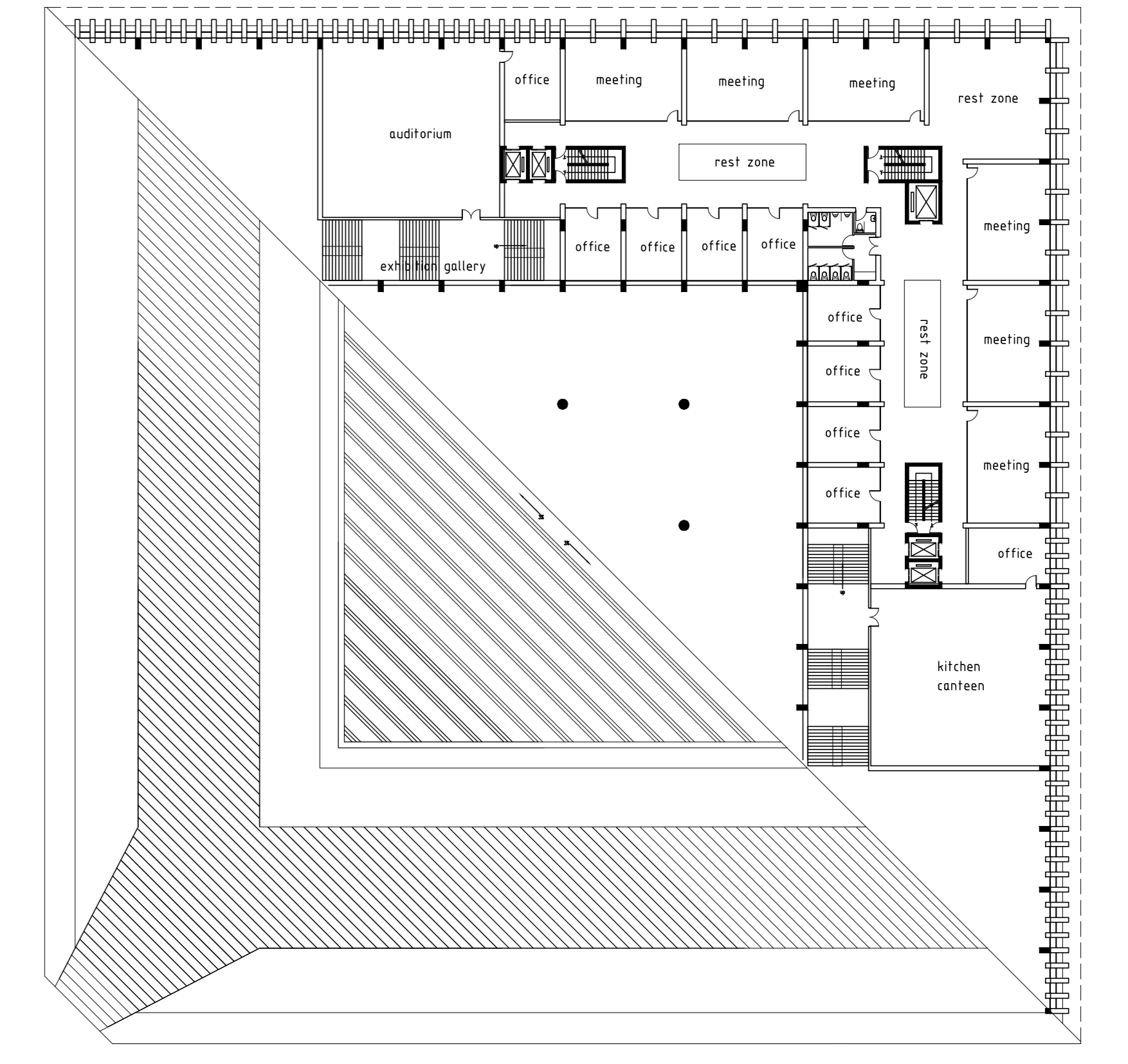
3 plan 1:200
