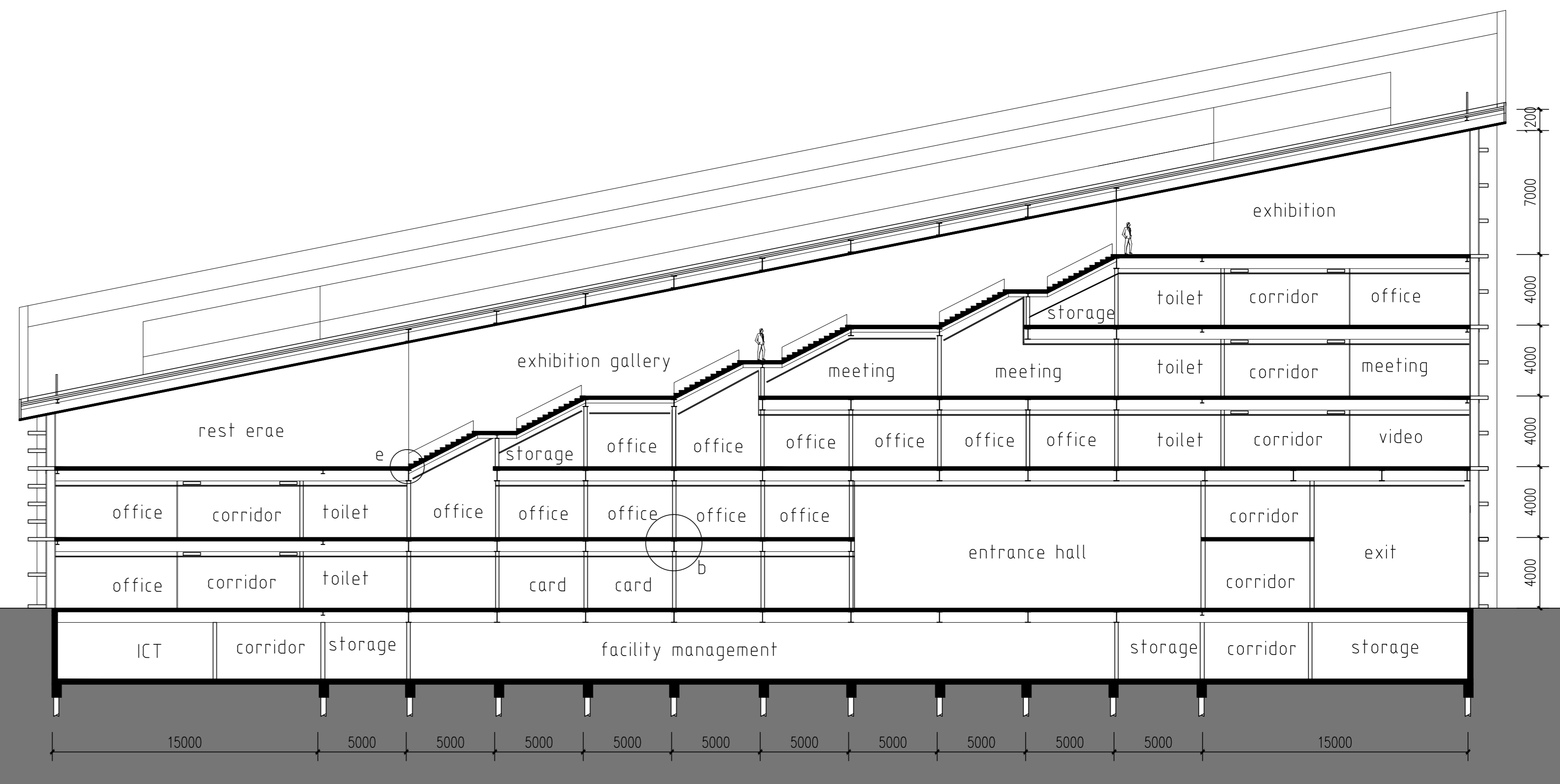
section 2-2 1:200
