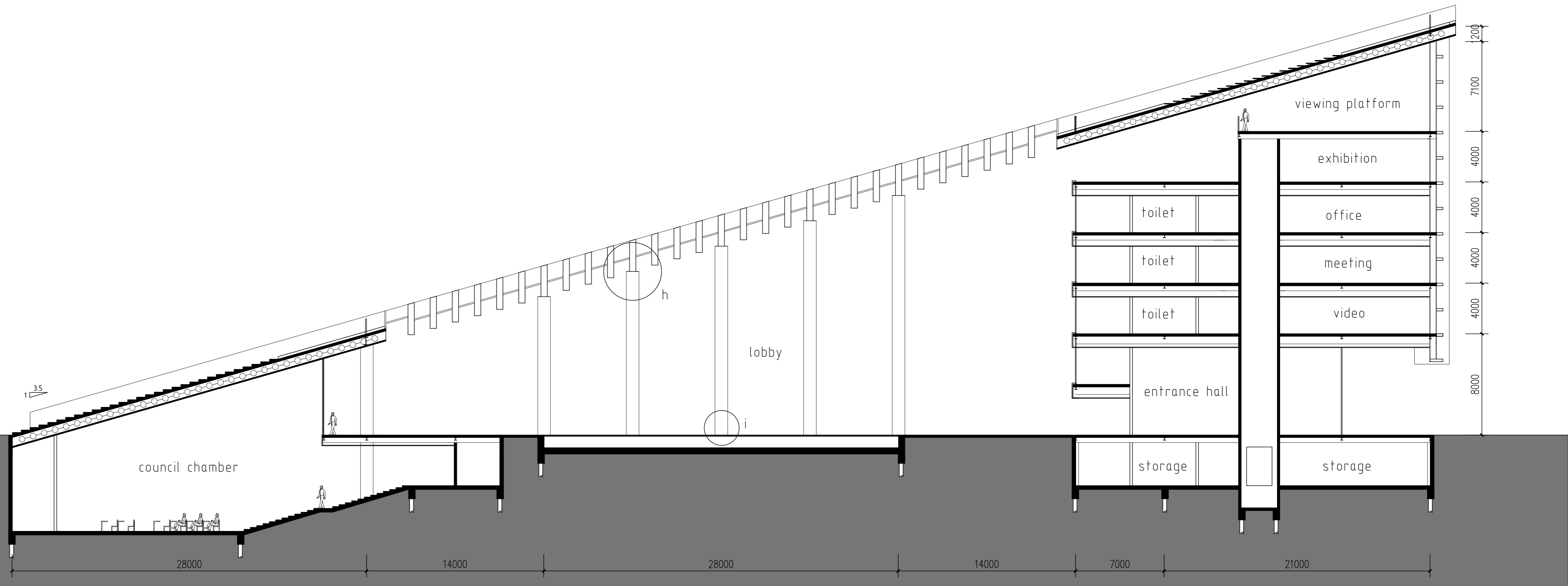
section 4-4 1:200
