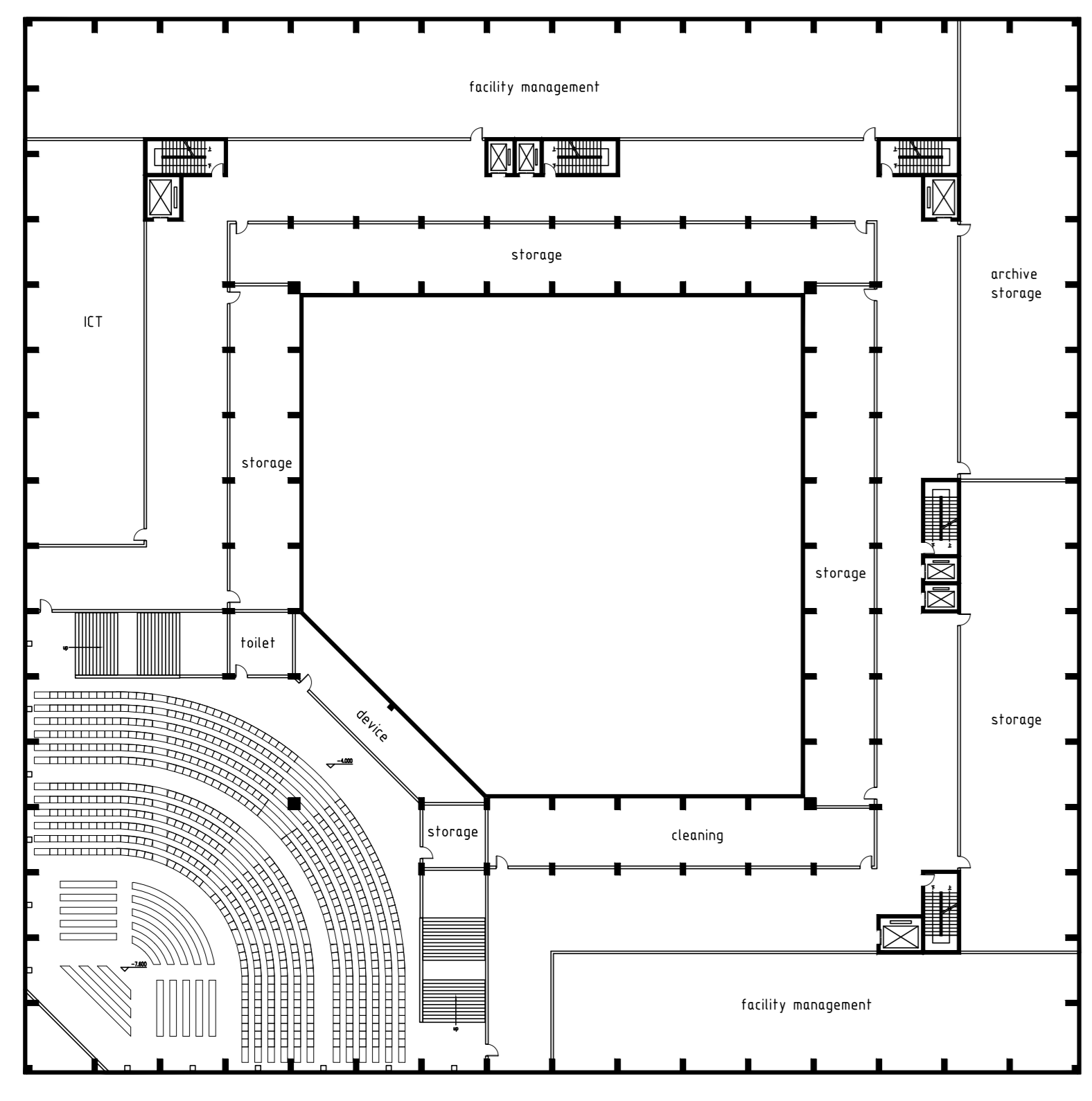
-1 plan 1:200
