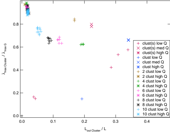
Fig. 6. Relative largest eigenvalue of the cluster \lambda_{max Cluster}/\lambda_{max G} as a function of the relative number of links leaving the cluster L_{out Cluster}/L for cluster network models.
