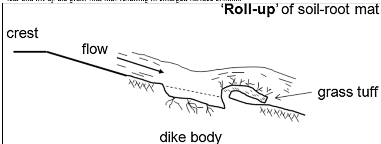
Fig. 3 Damage type ‘roll-up’, grass mat is cut underneath and pushed up gradually (after Hewlett et al. 1987)
