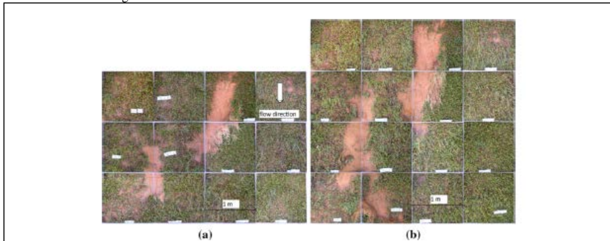
Fig. 2 Section Yen Binh YB4, surface erosion after (a) 2 h of 40 l/s per m + 6 h of 60 l/s per m + 4 h of 80 l/s per m and after (b) 2 h of 40 l/s per m + 6 h of 60 l/s per m + 6 h of 80 l/s per m + 6 h of 100 l/s per m
