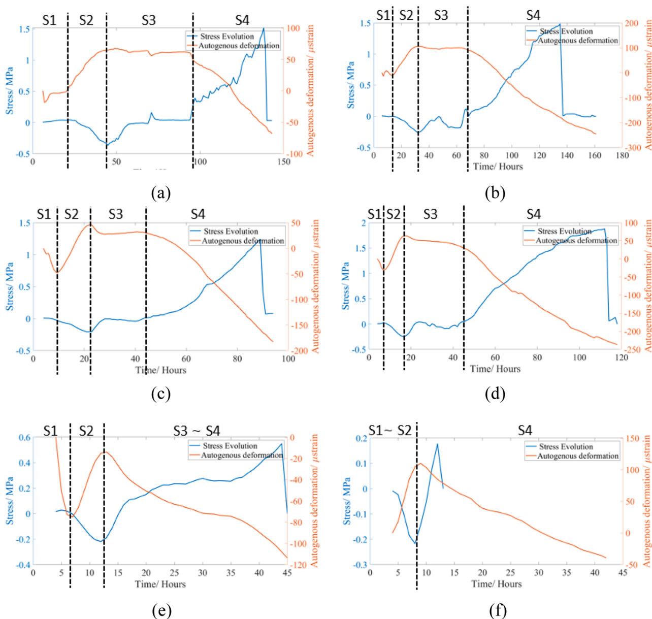
Fig. 7. The four-stage process of the AD and EAS evolution under six different temperatures: (a~ f) corresponds to the temperatures of 10 °C, 15 °C, 20 °C, 25 °C, 30 °C, and 40 °C respectively (Note that the scales of x-axis are different).
