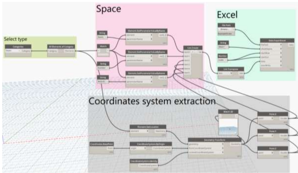
Figure 9: The Dynamo process flow that has been used to extract the location (xyz) of the spaces
