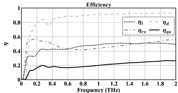
Fig. 1. Efficiency of the QO system: radiation efficiency of the lens antenna \eta_l (dotted line); reflectors system efficiency \eta_{rs} (dash-dotted line); detector efficiency \eta_d (dashed line); entire QO channel efficiency \eta_{qo} (solid line).
