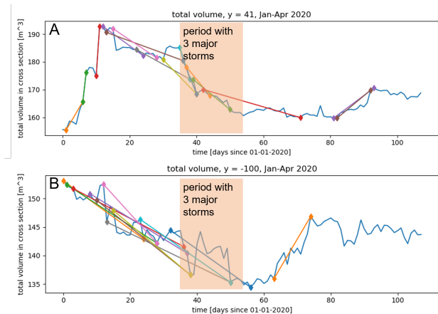
Figure 6. Time series of total volume in cross section cs1 (A) and cs2 (B) for January to April 2020. The threshold of volume change is set at absolute values greater than 10 \text{ m}^3 and all pairs of time stamps, between which the threshold is passed are marked with different colours.
