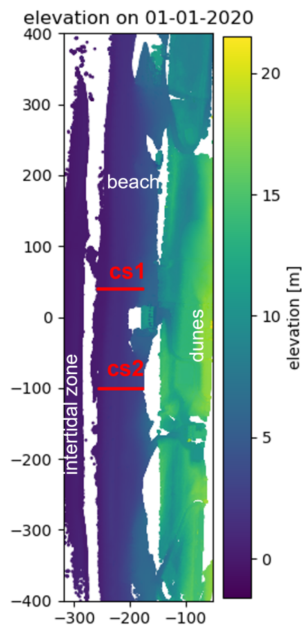
Figure 2. Location of cross section cs1 and cs2 marked in a point cloud of the observed area, covering the sandy beach, a part of the dunes and the intertidal zone in Noordwijk, The Netherlands.
