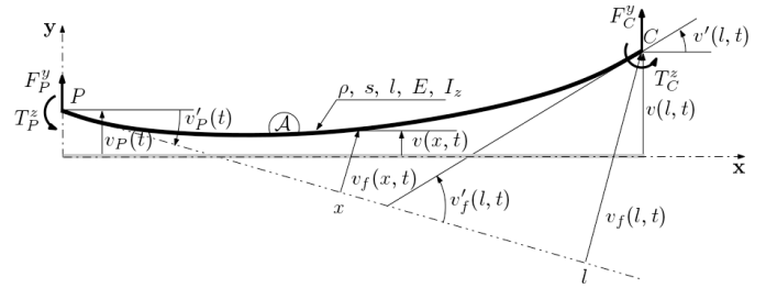
Fig. 1. Pure flexion (Alazard and Cumer (2018))
