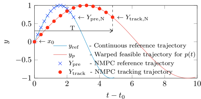
Fig. 1. Warping NMPC example with \dot{w}(t) = \frac{p(t)}{p_{\text{ref}}} = \frac{1}{2} .
