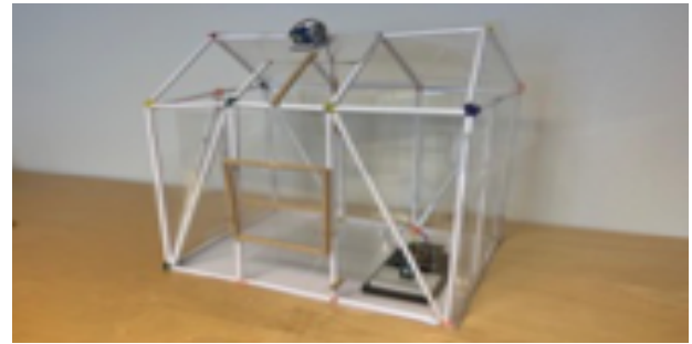
Figure 2. Vinyl/PVC build greenhouse.
