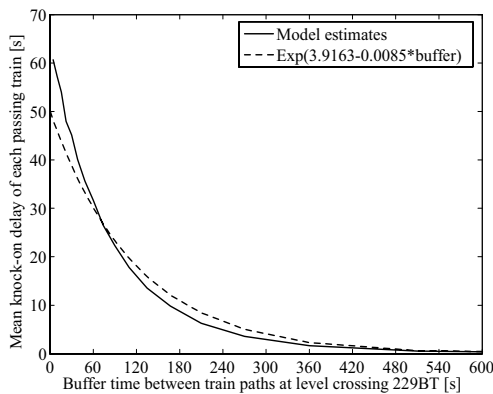
Figure 6.2: Mean knock-on delay as a function of buffer time between scheduled train paths at level crossing 229BT
