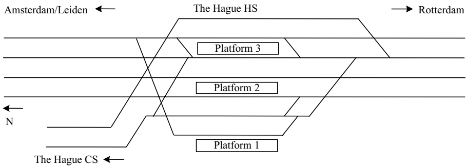
Figure 3.1: Scheme of railway network of The Hague HS station
