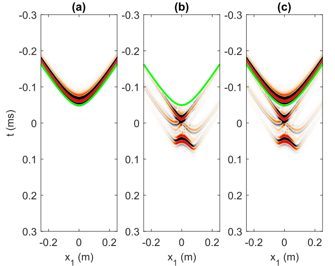
Fig. 5. (a) Direct focusing function F_{Ud} . (b) Coda of the focusing function F_{Um} as retrieved by solving the Marchenko equation under the direct-wave approximation F_{Ua} = 0 . (c) Updated focusing function F_U , as obtained by adding the retrieved coda F_{Um} to F_{Ud} . All panels are clipped at 10% of the maximum amplitude of the direct wave.
