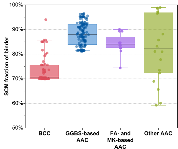
Fig. 1 SCM fractions of the binders of the mixes included in the database. ‘Binder’ refers to the solid starting materials and the oxides ( \text{Na}_2\text{O} , \text{SiO}_2 etc.) dissolved in the activator solution combined. Twenty additional blended-cement concretes/mortars (BBC) based on CEM III/B (66–80% GGBS in binder) are not included in the plot. Black lines represent the medians; boxes represent the ranges between the 25% percentile and the 75% percentile; and the whiskers represent the 5% percentiles and the 95% percentiles
