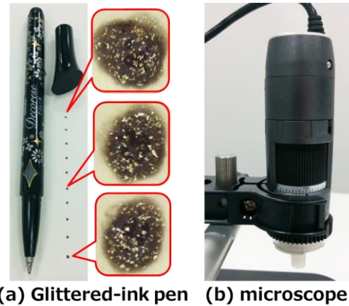
Figure 4: Hardware components and mIDoT images dotted and captured by them; (a) glitter ink pen for marking unit, (b) microscope for capturing unit.
