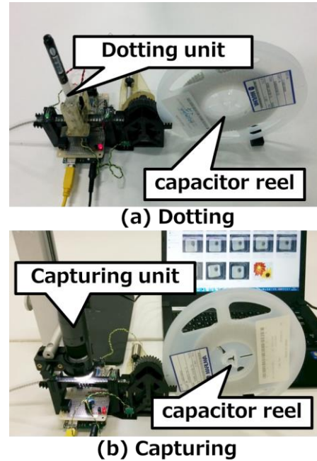
Figure 2: the overview of Tip-on-a-chip system; (a) dotting, (b) capturing
