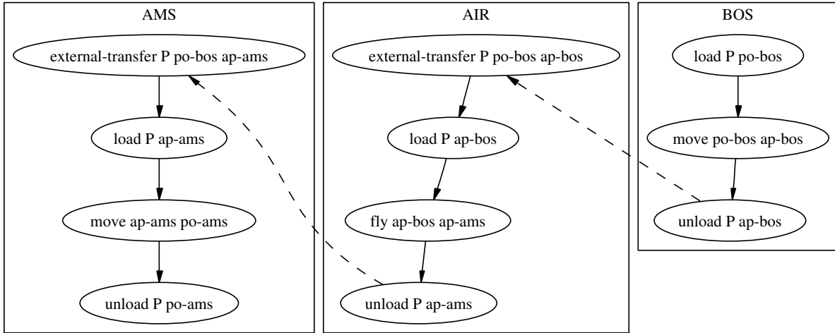
Figure 1: The multiagent plan for transporting package P from po-bos to po-ams using three agents: BOS, AIR, and AMS.
