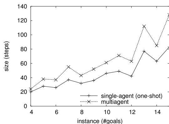
Figure 5: Plan lengths of single-agent one-shot planning, and the cumulative size of the multiagent plans.
