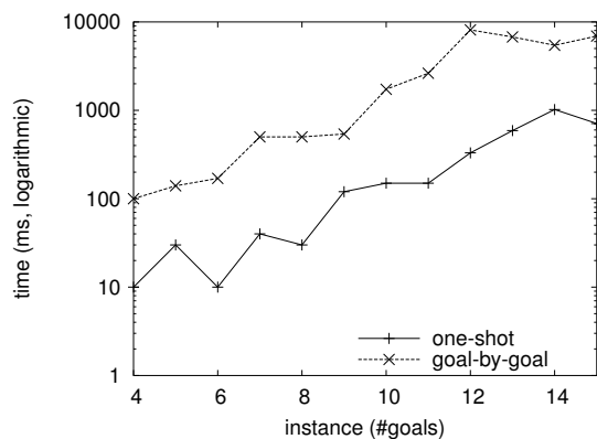
Figure 2: Run times of one-shot planning and goal-by-goal planning by a single agent.
