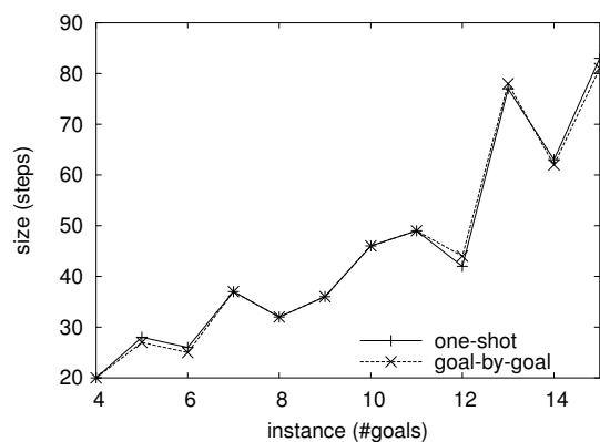
Figure 3: Plan lengths of one-shot planning and goal-by-goal planning by a single agent.
