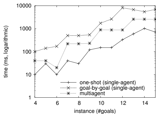
Figure 4: Run times of multiagent planning compared to single-agent planning. The time reported for the multiagent experiments is the time it took the slowest of the agents to compute its plan (the “make span”).
