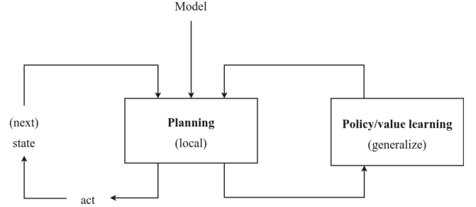
Figure 1: Multi-step Real-time Dynamic Programming. The three key procedures are 1) Planning, 2) Learning, and 3) Real steps (acting).
