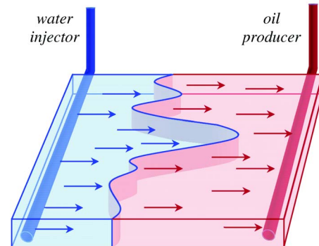
Fig. 1. Process of water flooding using a (horizontal) injection and production well. The irregular-shaped oil-water front is a result of the heterogeneous nature of the reservoir (after [2]).
