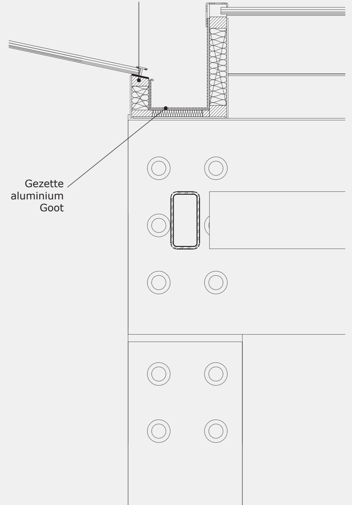
Detail 3 1:5
