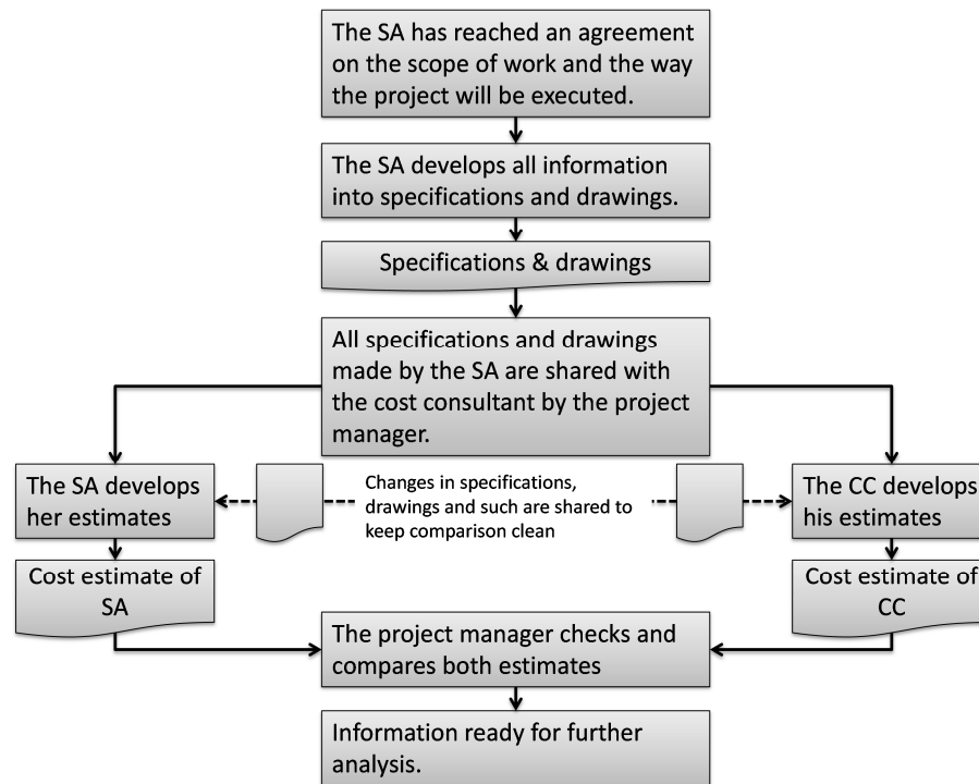
Figure 2. Method followed to get comparable estimates from the SA and CC
