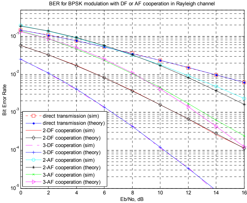
Figure 7. BER performance for DF or AF cooperation.
