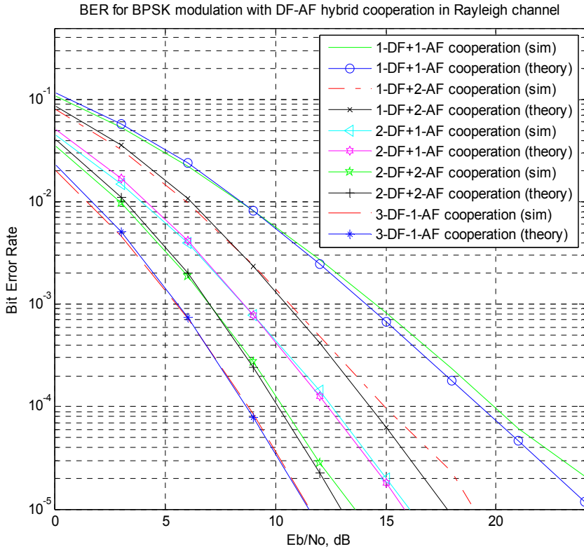
Figure 8. BER performance for hybrid DF+AF cooperation.
