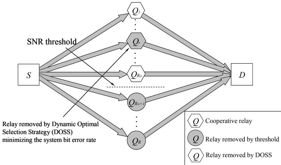
Figure 4. Cooperative wavelet communication scheme with dynamic optimal selection of DF relays in wideband multi-scale and multi-lag channel ( S : Source, D : Destination, Q : r -th Relay).
