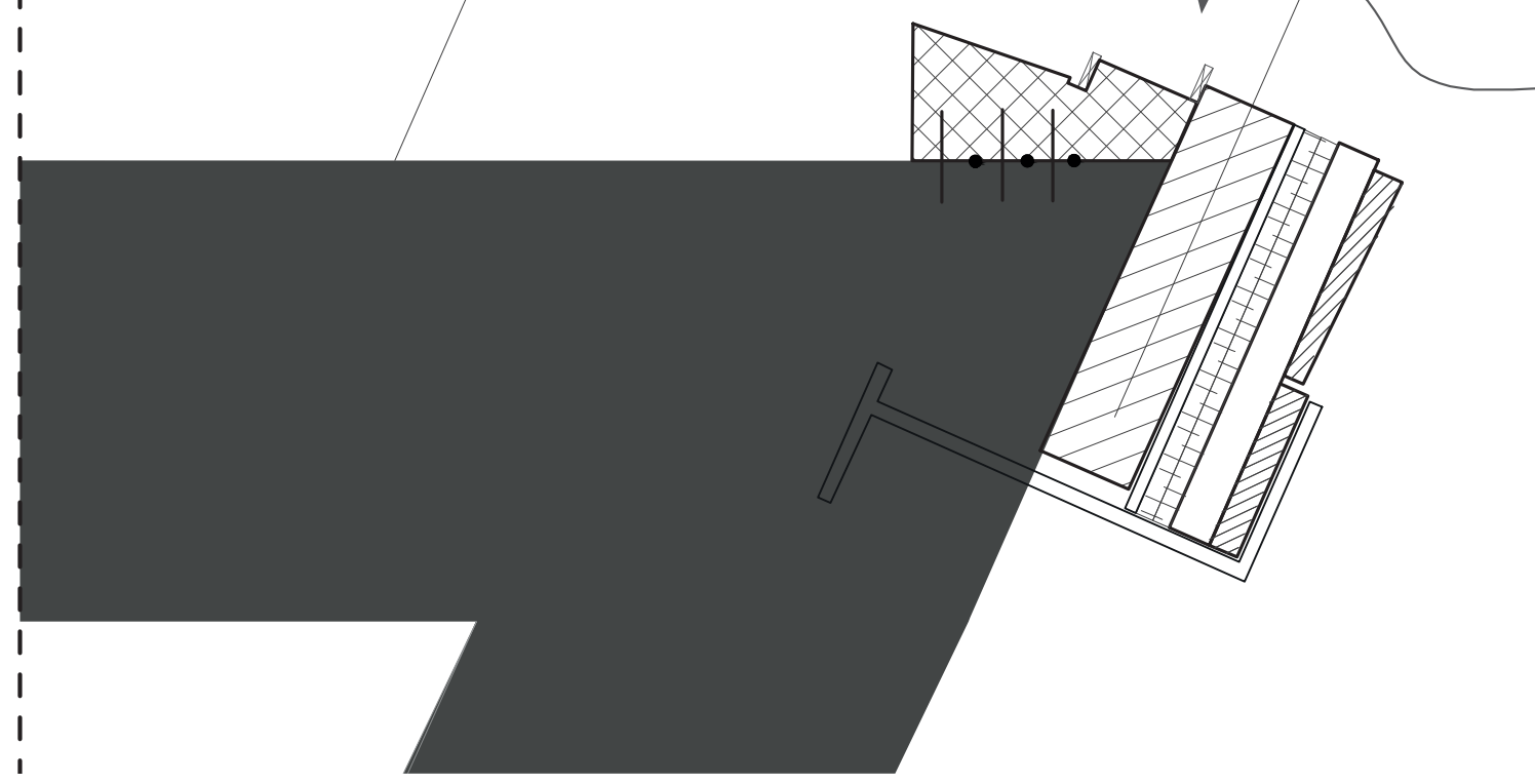
detail 6 vertical | scale 1:5 connection floor
