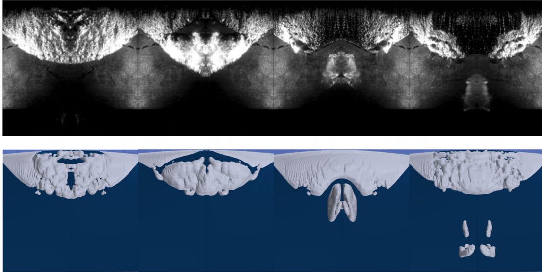
Fig. 19 Qualitative comparison between the particle image velocimetry imaging and the simulated shedding cycle, visualized as an isosurface of \alpha_v = 0.01
