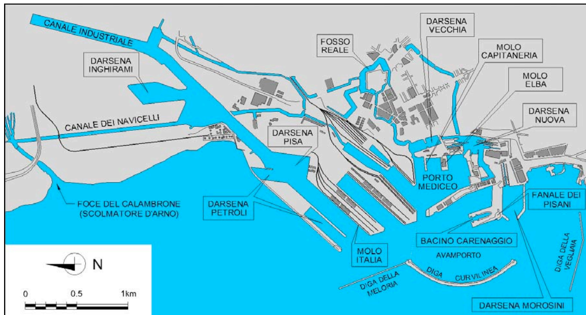
Figure 10. 1953 Port Plan.
