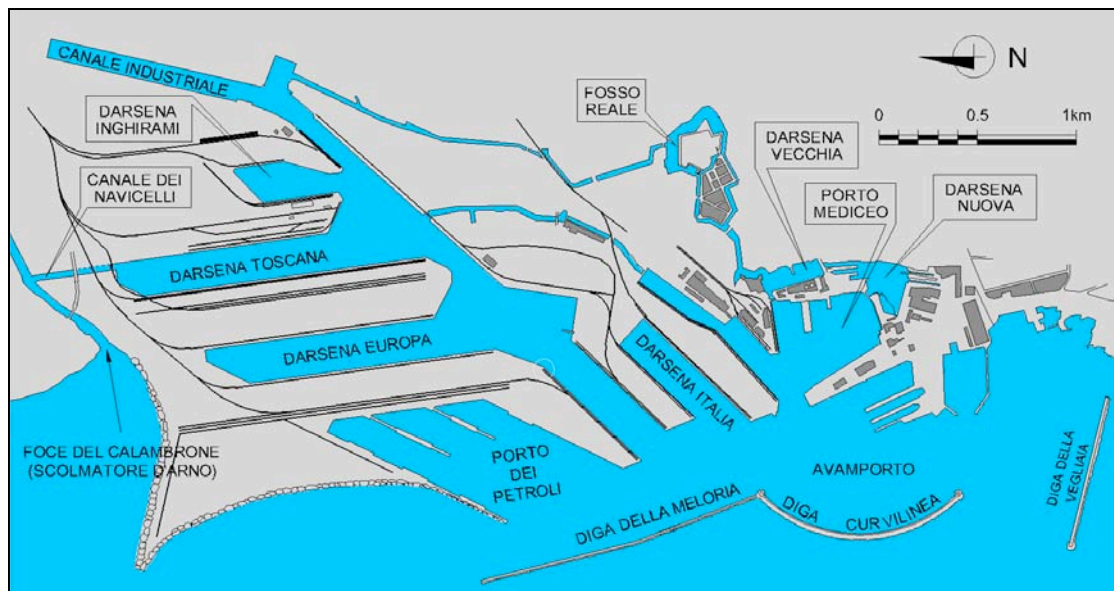
Figure 12. Port Plan proposed in 1971.
