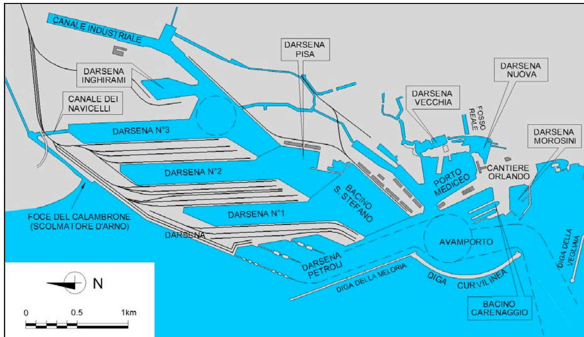
Figure 11. Final Proposal of the Committee chaired by Eng. P. Vian (1965.)
