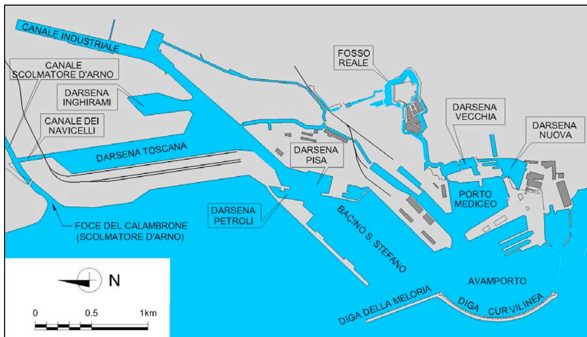
Figure 13. Variant of the 1953 Port Plan proposed in 1973.
