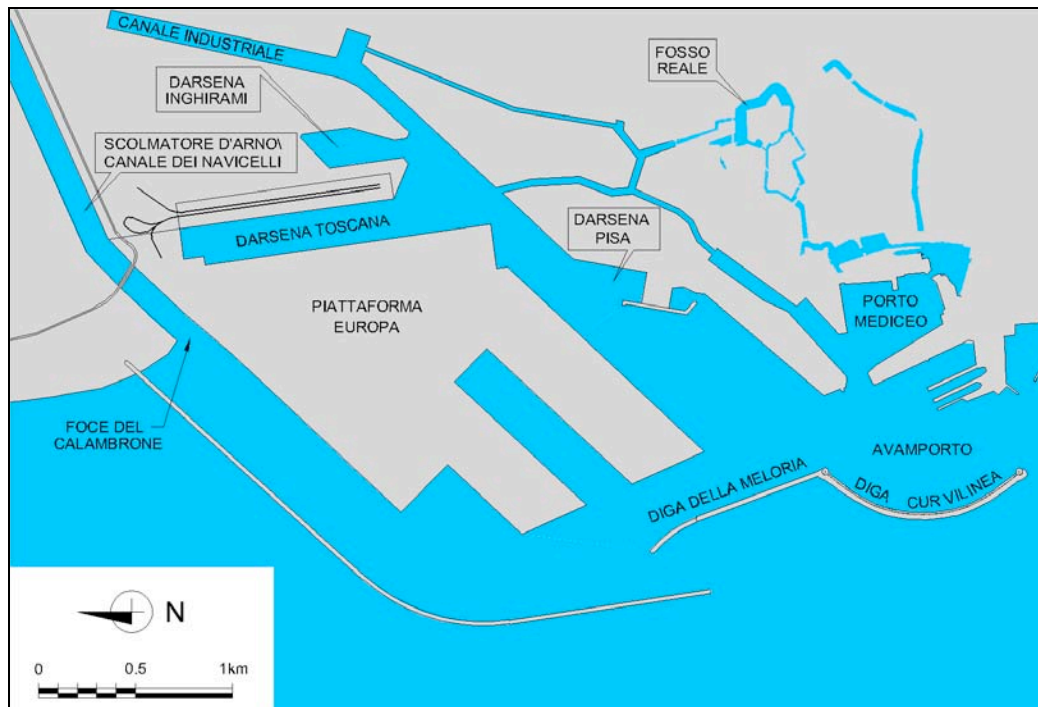
Figure 14. Port Plan proposed by Bonifica (1980).
