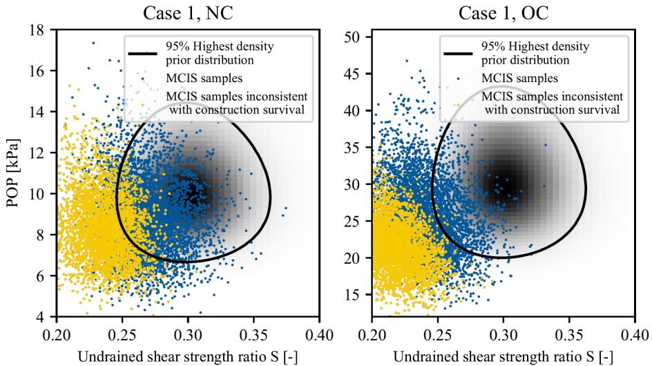
Figure 4.6: Joint probability density (grey shading) for undrained shear strength ratio ( S ) and POP values. Blue dots show all MCIS samples, yellow dots show only realisations that are not consistent with the survived construction (i.e. for which h(\mathbf{x}_{s,i}) > 0 ).
