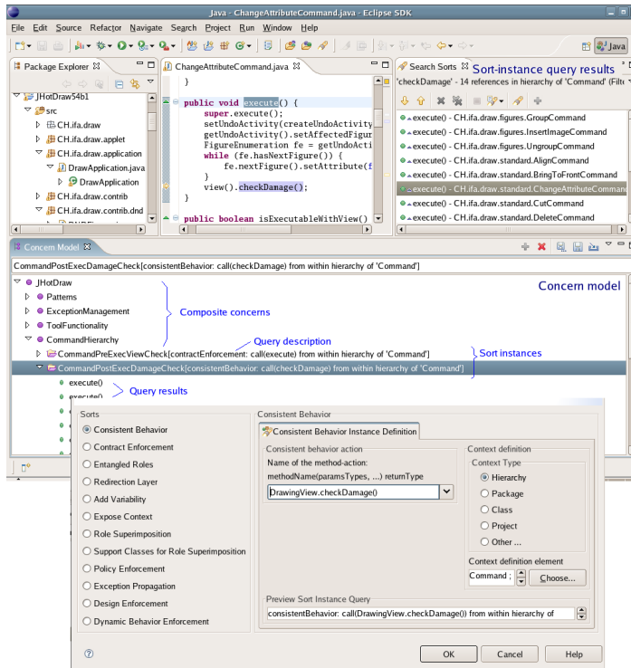
Figure 1. SoQuET views and dialogs
