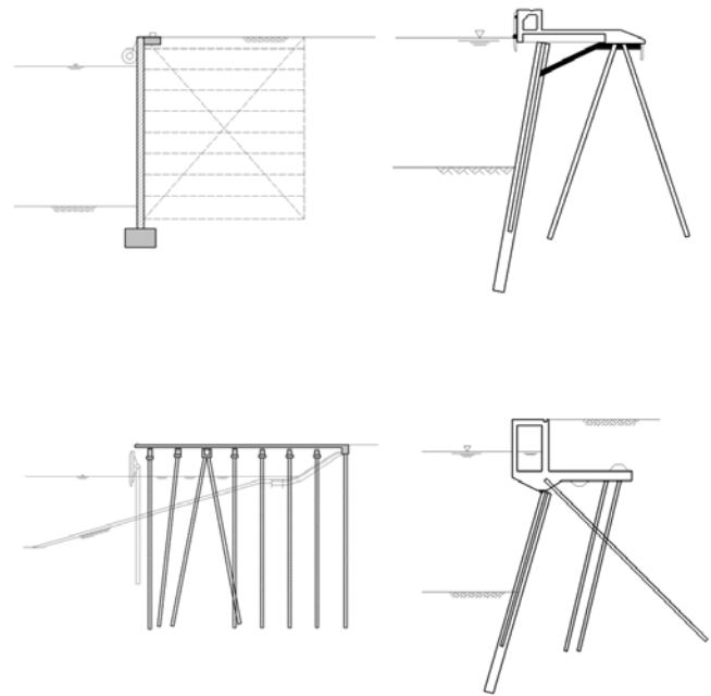
Figure 1 Examples of quay wall structure and super structure types covered by the IfcQuay domain model extension of the Industry Foundation Classes model
