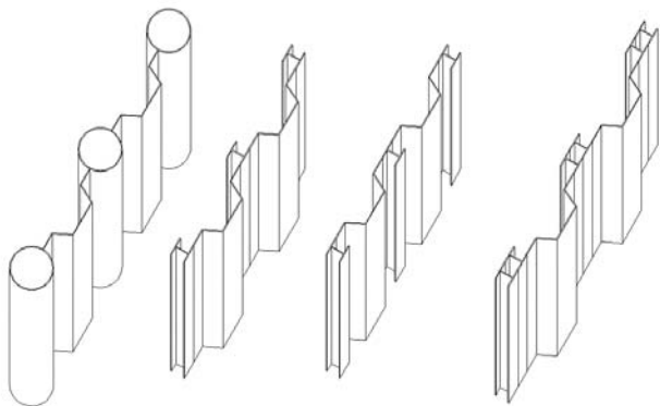
Figure 2 examples commonly employed retaining wall structures captured as parametric geometries in IfcQuay
