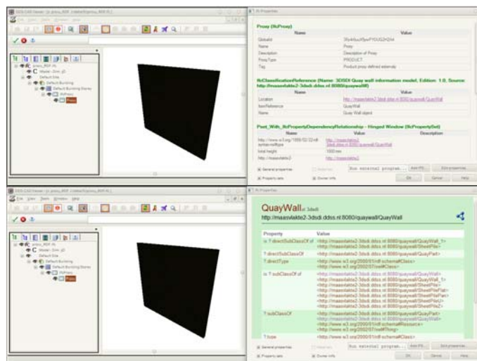
Figure 5 Unmodified, off the shelf legacy software application (DDS CAD) displaying properties of an IfcProxy object that has been enriched with RDF vocabularies
