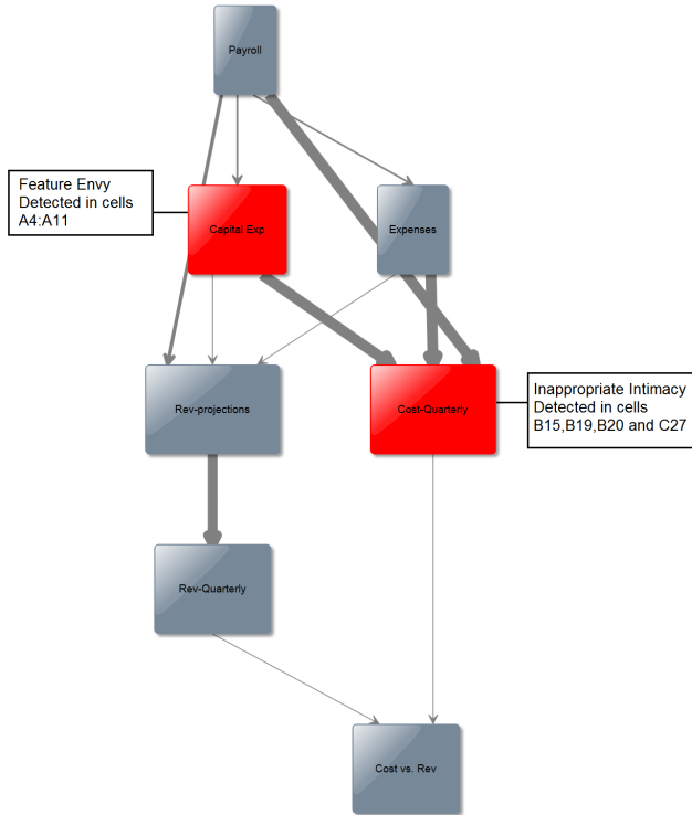
Figure 3. A screenshot of a spreadsheet data flow visualization enriched with smell information
