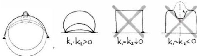
Figure 6: Principles for designing pneumatic formworks [8]
