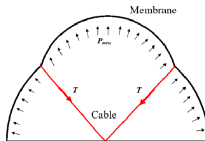
Figure 12: The force diagram of the cable and the membrane by adding internal cables
