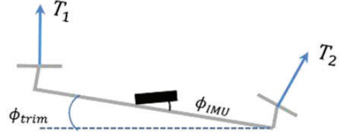
Figure 2. When a quadrotor hovers, usually the average attitude of the quadrotor and reading of the AHRS are not zero. This is caused by the misalignment of both the IMU and the rotors.
