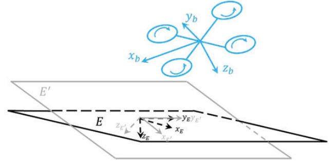
Figure 4. AHRS estimation errors can be represented by an erroneous Earth reference frame E' .
