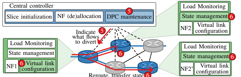
(c) Interactions between components during scaling-out. DPCs continuously track the slice's utilization (step 1, Sec. II-A). If they detect overload, they notify the CC (step 2). The CC subsequently determines the switch where NF2' will be deployed on and the route to connect the node to the rest of the slice (step 3). Next, the CC deploys the new NF (step 4) and, upon its completion, informs NF1 to divert a portion of its traffic to the newly deployed NF2' (step 5). When a packet of this flow is received, the state from NF2 is transferred to NF2', and a virtual link is created using the Slice Management Protocol (step 6, Sec II-B).
