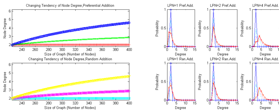
Figure 4.6.1 (a) Left: Evolving node degree, in line graph (b) Right: Evolving node distribution, in line graph
