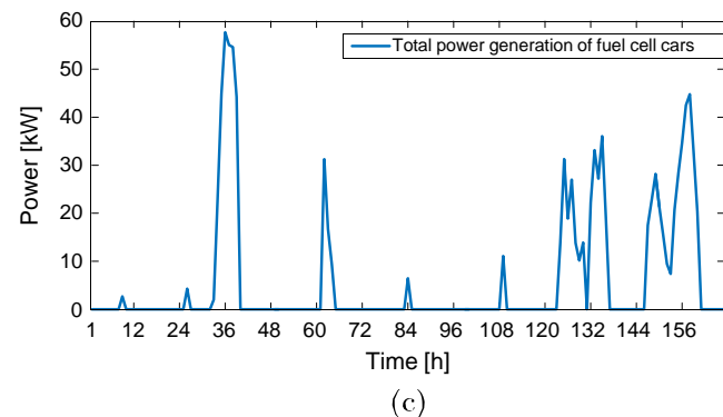
Fig. 5. Operation of the control system during a week. (a) Imported power to the microgrid from the power grid. The red dashed lines indicate the limits on the exchanged power between the power grid and the microgrid. (b) Electrical power usage of the water electrolysis system. (c) Total power generation of fuel cell cars.
