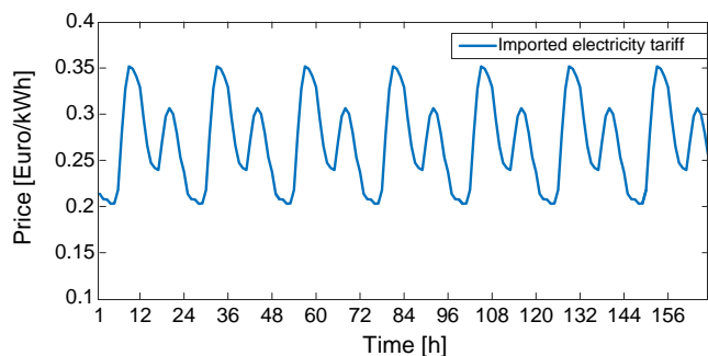
Fig. 3. Price of importing electricity to the microgrid based on the APX market.
