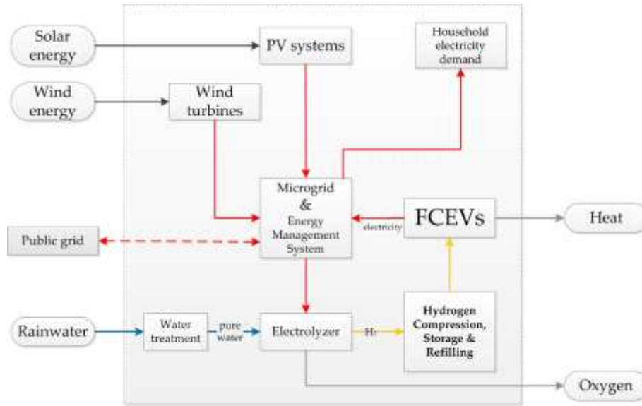
Fig. 1. Schematic presentation of the CaPP microgrid system.
