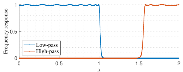
Fig. 1: Illustration of a high-pass graph filter obtained by transforming the low-pass counterpart via Algorithm 2. The high-pass filter requirements are \tilde{\delta}_p = \tilde{\delta}_s = 0.01 ; \tilde{\lambda}_p = 1.575 , \tilde{\lambda}_s = 1.425 .
