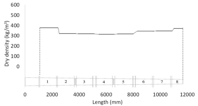
Figure 8. Dry density profile (for a m.c. of 0%) of a full-length pile divided in 8 segments.
