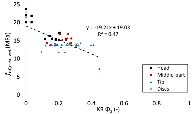
Figure 6. Correlation between f_{c,0,meas,wet} and KR calculated with \Phi_2 for pile segments divided in head, middle-part and tip, and discs.
